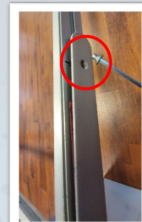
4: put in the screws (4 screws)
