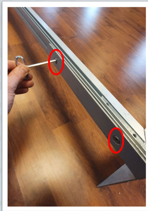
2: take out the screws at the side (4 screws)
